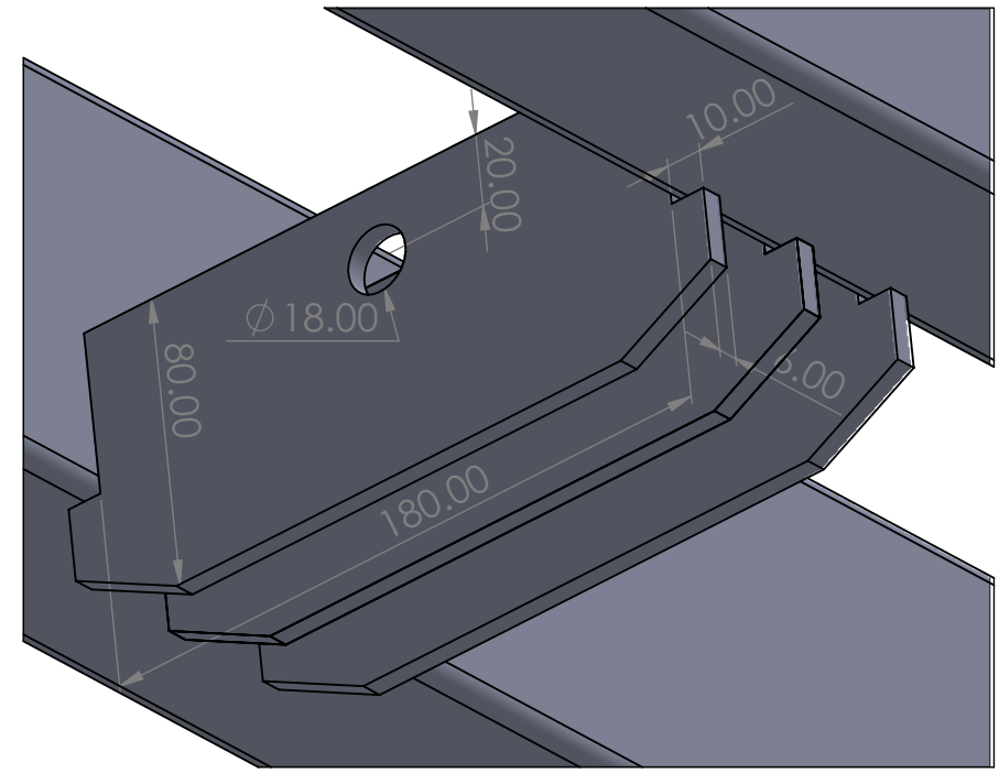
Detail showing Cylinder Mount
