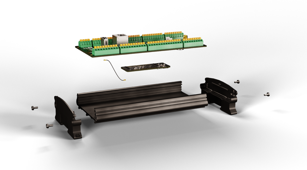
The Portenta Machine control exploded view
