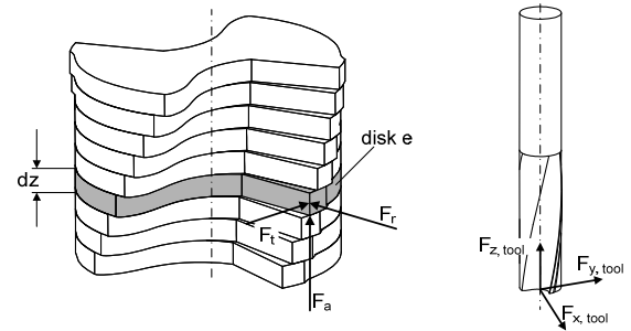
FIGURE 7. Resulting force on the TCP.
